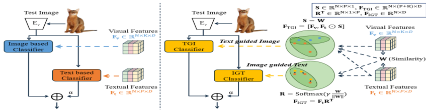
Figure: TIMO Architecture Overview
